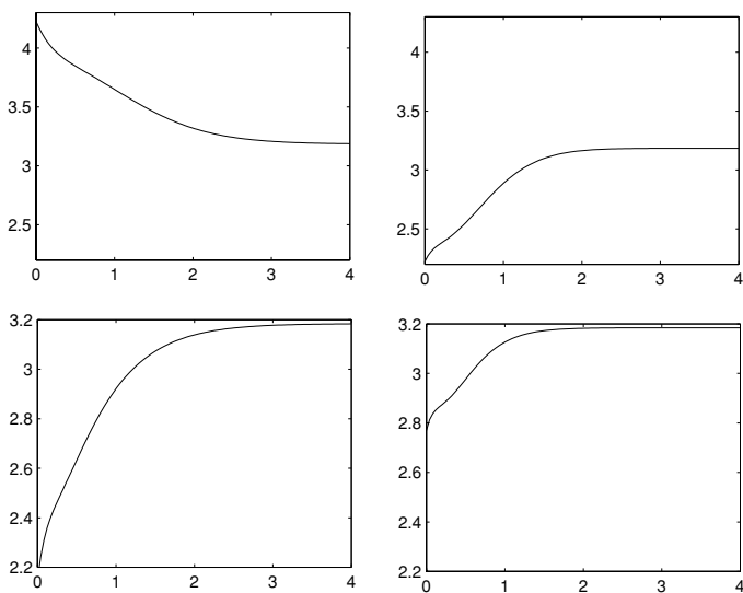
Fig. 1. Entropy behavior for the overdamped noisy harmonic oscillator when \alpha_1\alpha_2 \geq 0 . The left hand panels show plots of H_G(P^t f_0) as a function of time as given by Eq. (4.29) and the right hand panels show H_{NE}(P^t f_0) \equiv H_C(P^t f_0|f_*) + H_G(f_*) as a function of time. The parameters used were m = 1 , \gamma = 3 , \omega^2 = 2 , and \sigma_* = 1 . Upper panels correspond to the range of parameters as in Eq. (A.5) with specific values \bar{\sigma}_1 = 2 , \bar{\sigma}_2 = 2 , while the lower panels correspond to parameters as in Eq. (A.10) with \bar{\sigma}_1 = 0.5 , \bar{\sigma}_2 = 1 .
